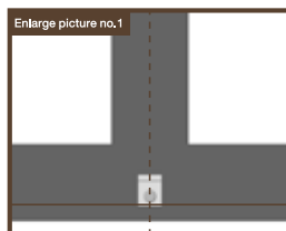
Attach clip lock at indicated height and in the center of steel frame.
